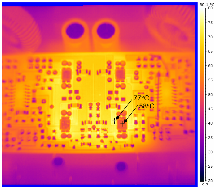
Thermal image of daughter board running at 2\text{ch} \times 1/8^{\text{th}} rated power - steady state, T_c < 58^\circ\text{C}
